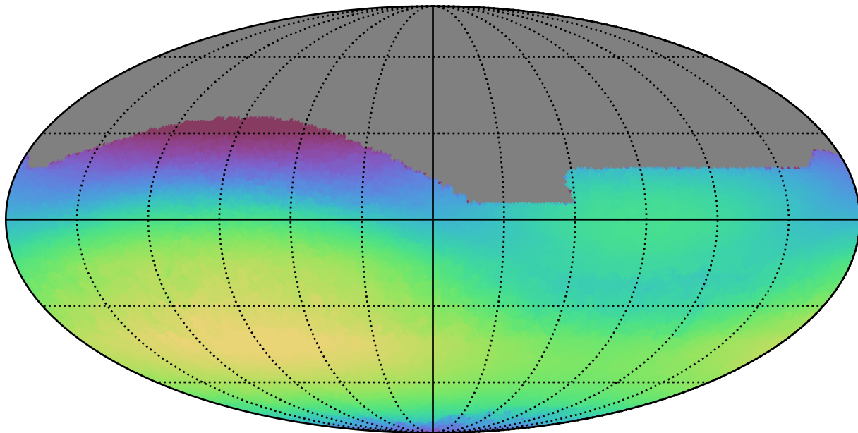
too_5_1v3.4_10yrs All sky r band: Max skyBrightness
