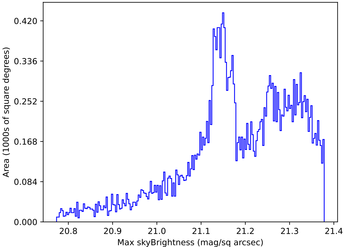
too_5_1v3.4_10yrs All sky r band: Max skyBrightness
