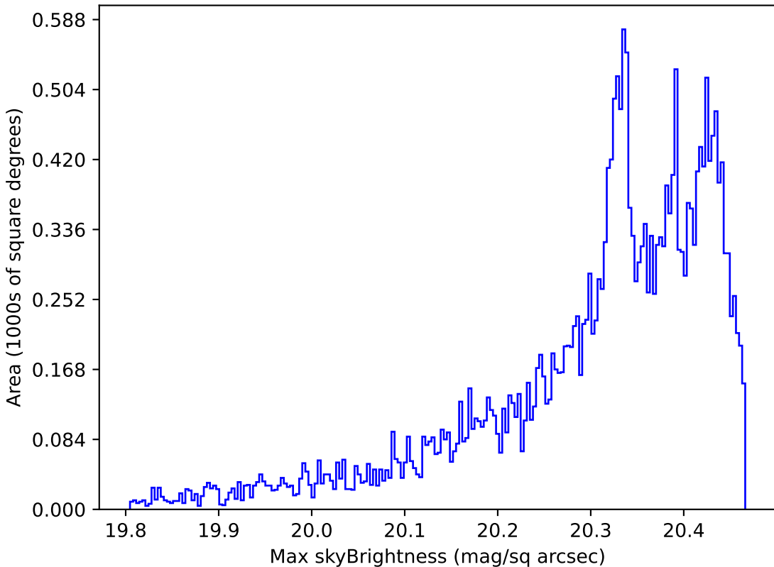
too_5_1v3.4_10yrs All sky i band: Max skyBrightness
