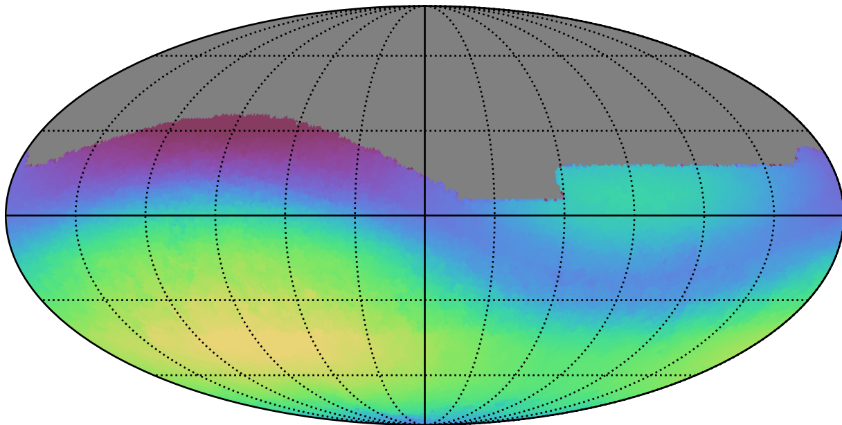
too_5_1v3.4_10yrs All sky g band: Max skyBrightness
