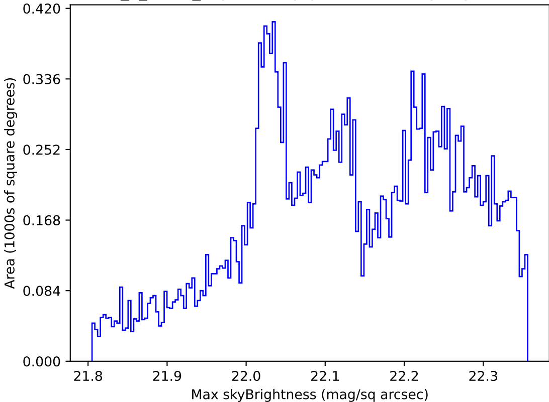
too_5_1v3.4_10yrs All sky g band: Max skyBrightness
