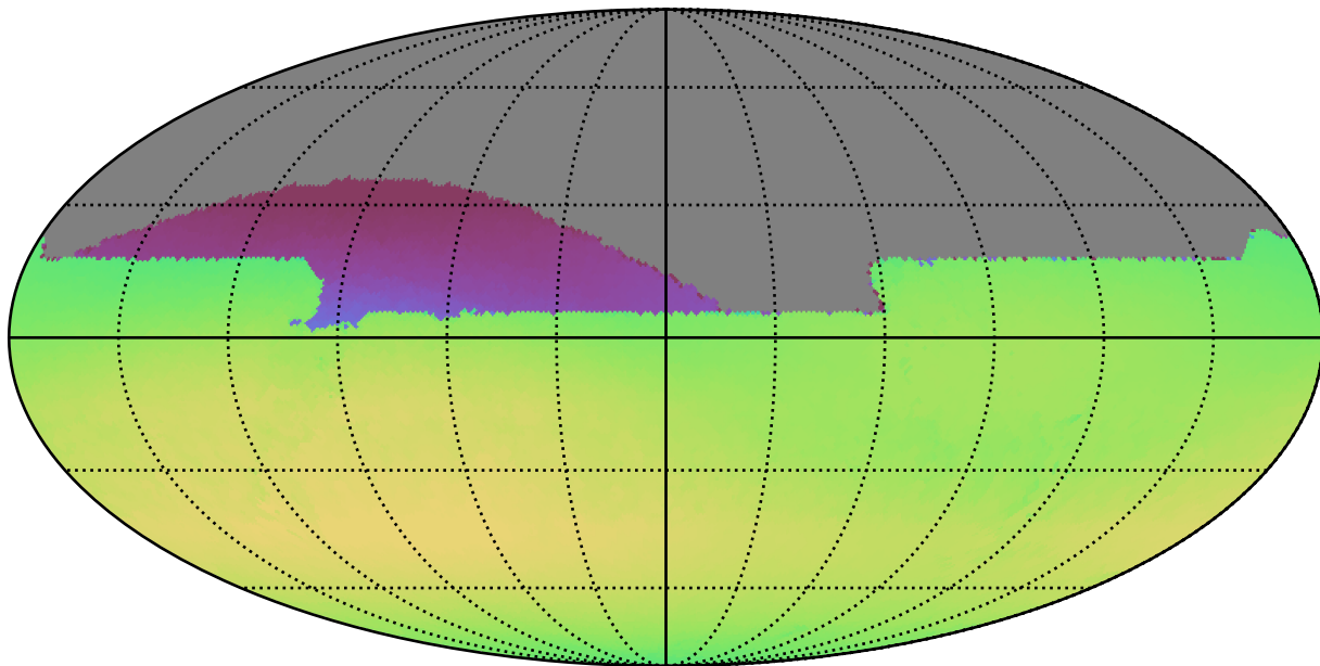
too_5_1v3.4_10yrs All sky all bands: Max skyBrightness
