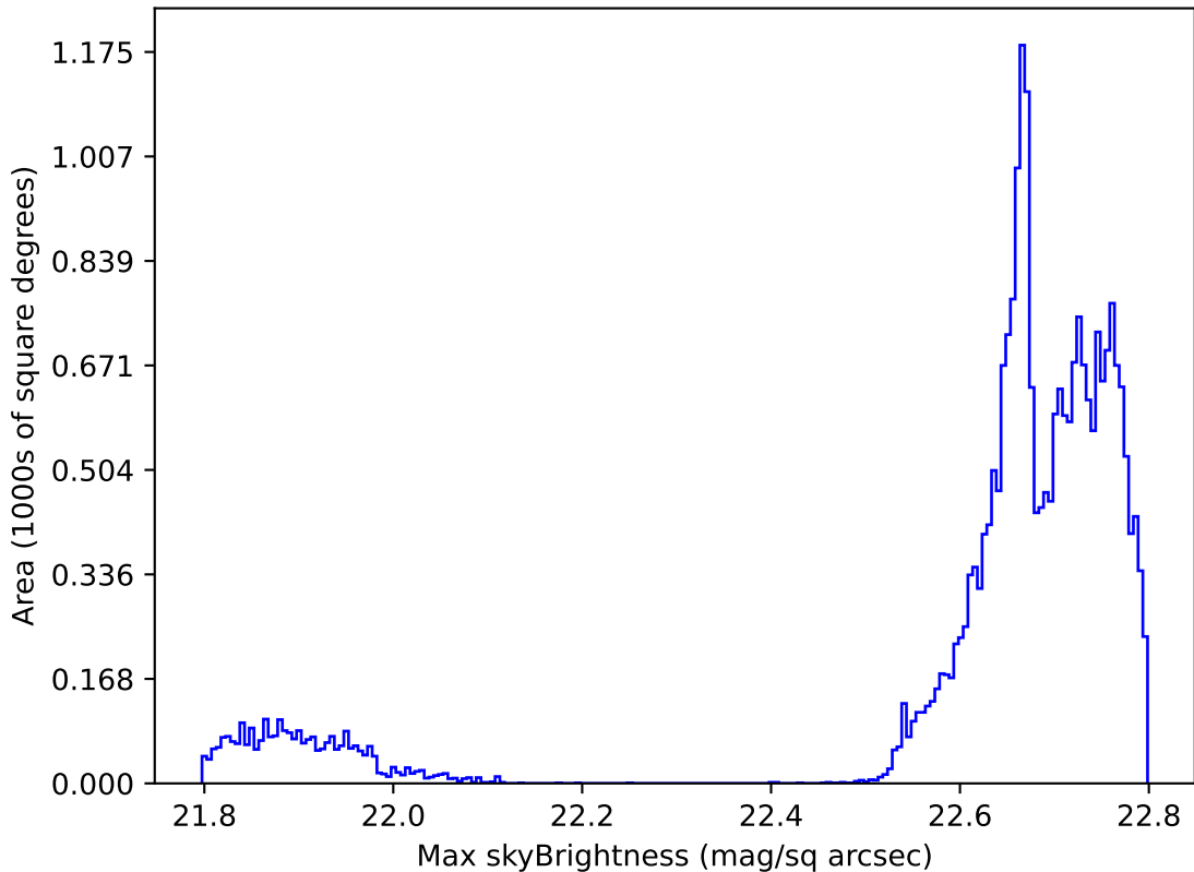
too_5_1v3.4_10yrs All sky all bands: Max skyBrightness
