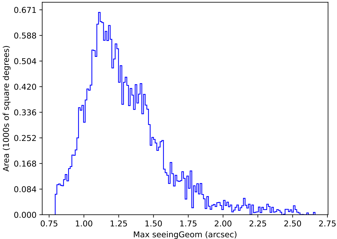
too_5_1v3.4_10yrs Yr 1 z band: Max seeingGeom
