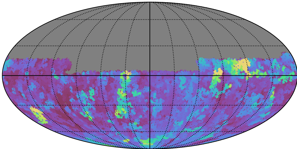
too_5_1v3.4_10yrs Yr 1 u band: Max seeingGeom
