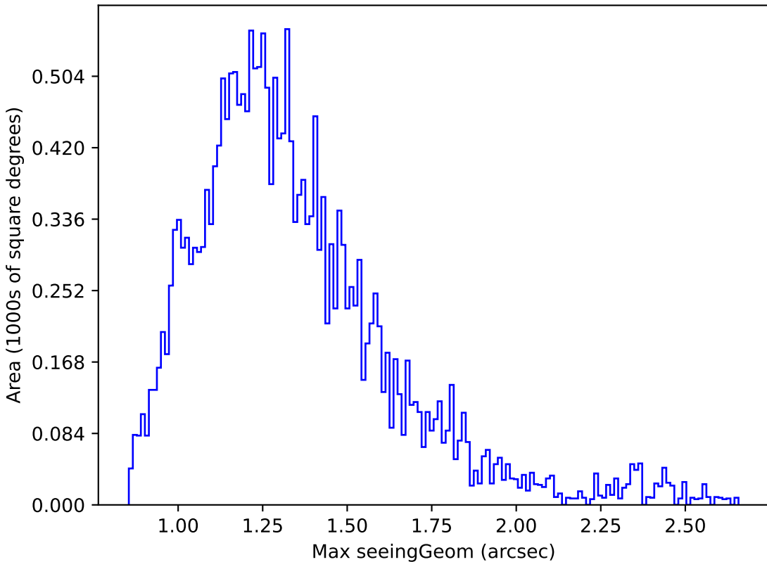
too_5_1v3.4_10yrs Yr 1 u band: Max seeingGeom
