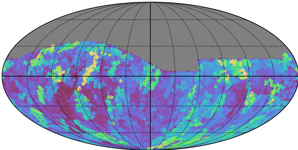
too_5_1v3.4_10yrs Yr 1 r band: Max seeingGeom
