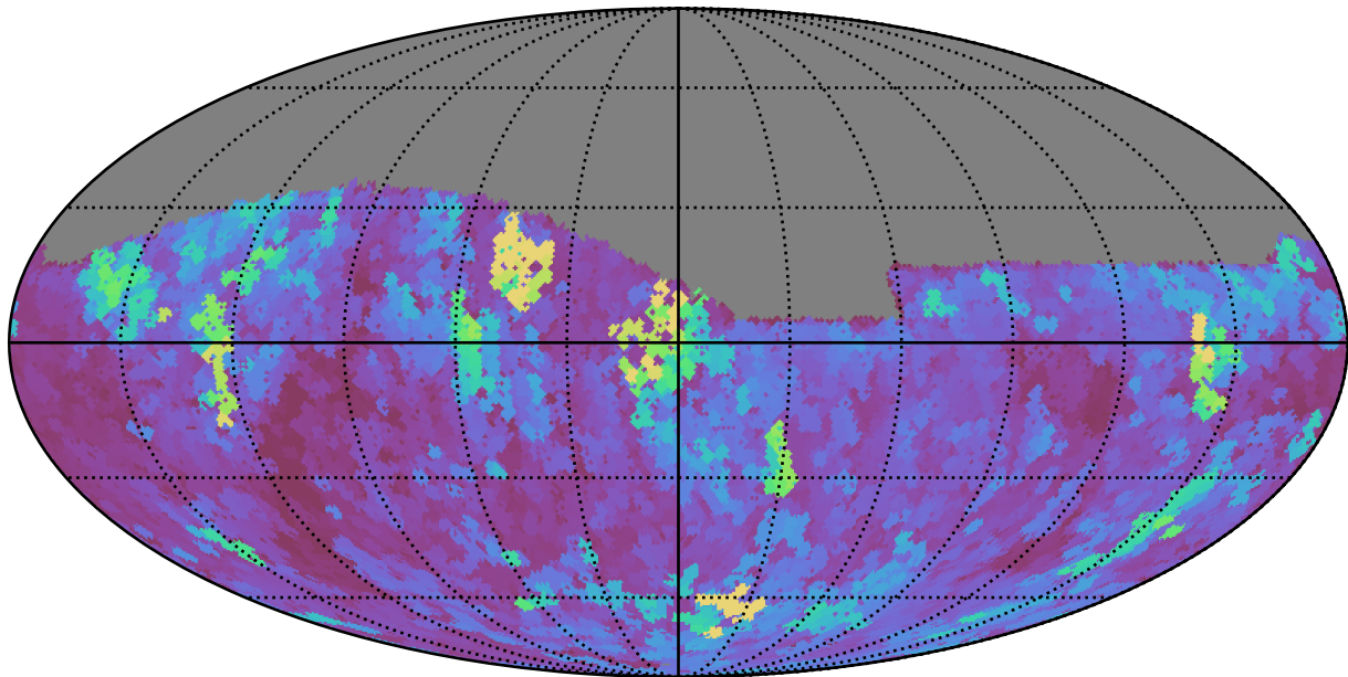
too_5_1v3.4_10yrs Yr 1 i band: Max seeingGeom
