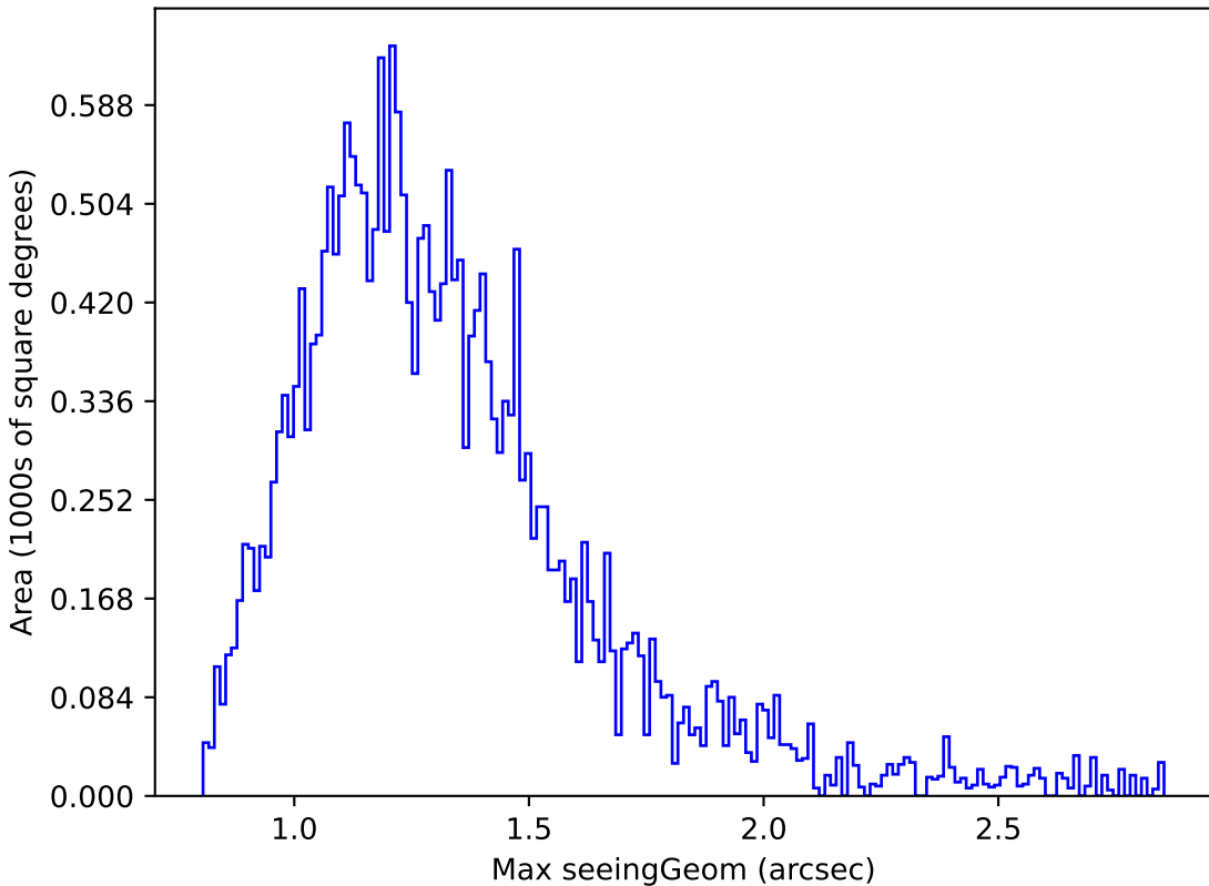
too_5_1v3.4_10yrs Yr 1 i band: Max seeingGeom
