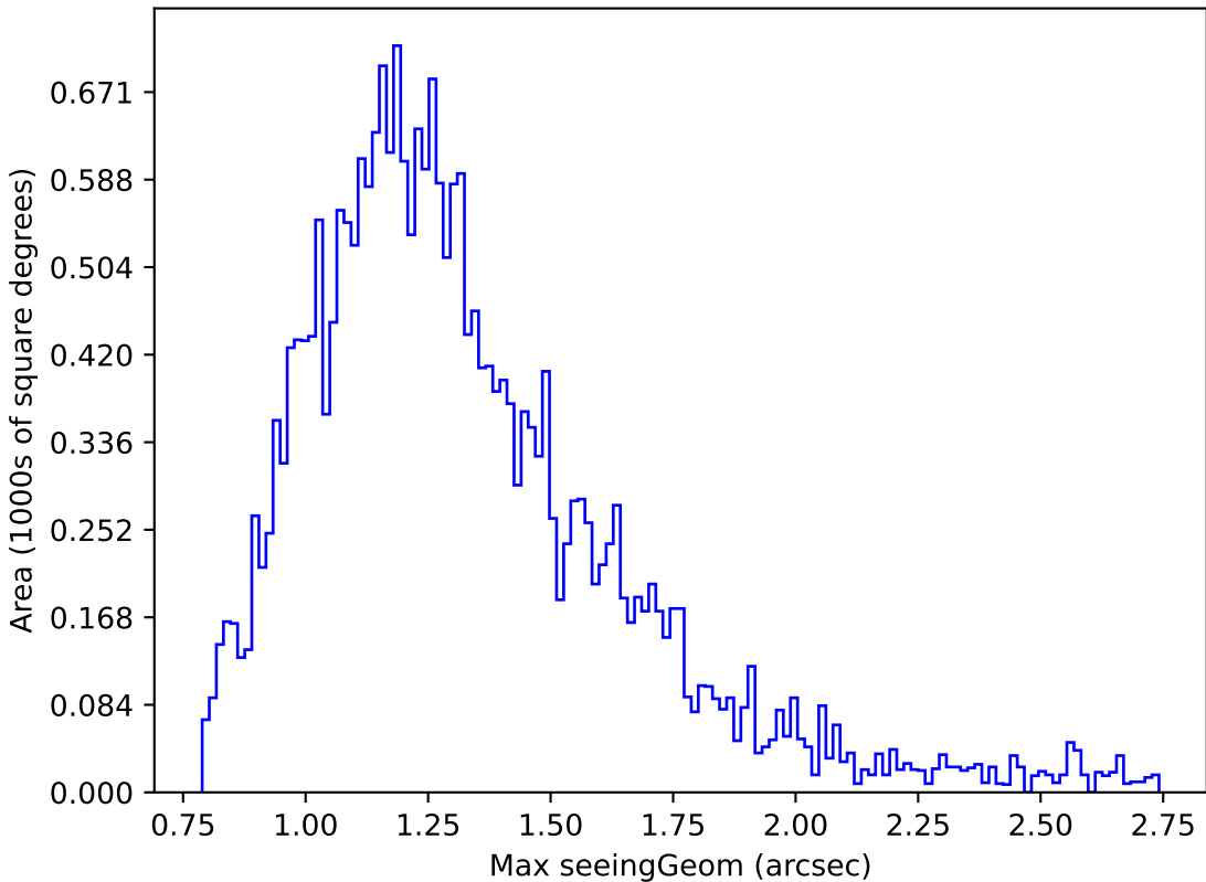
too_5_1v3.4_10yrs Yr 1 g band: Max seeingGeom
