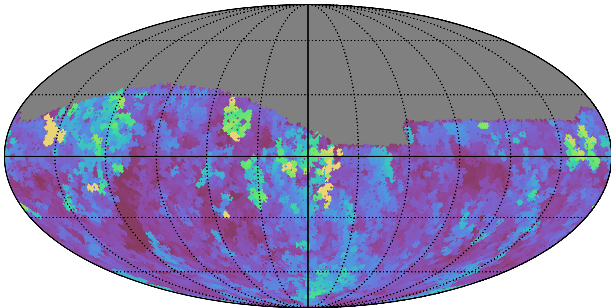
too_5_1v3.4_10yrs Yr 1 z band: Max seeingEff
