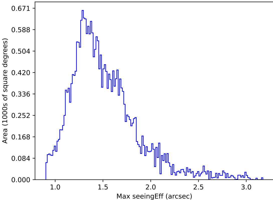
too_5_1v3.4_10yrs Yr 1 z band: Max seeingEff
