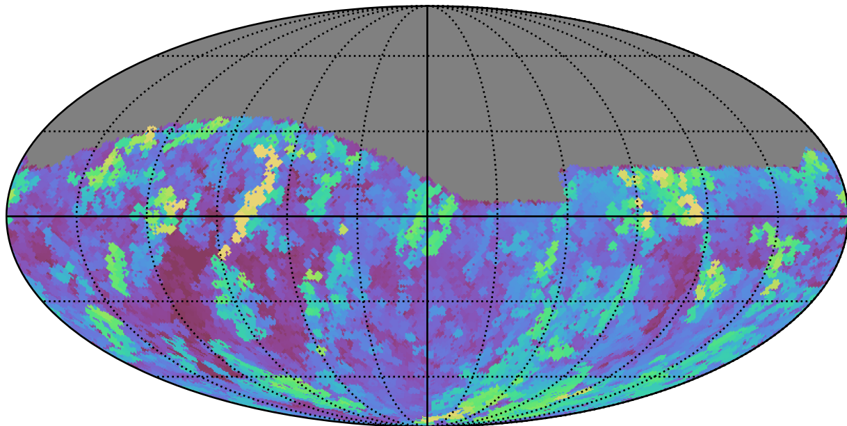
too_5_1v3.4_10yrs Yr 1 r band: Max seeingEff
