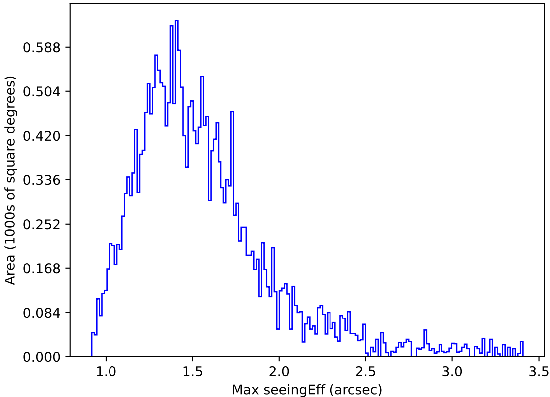
too_5_1v3.4_10yrs Yr 1 i band: Max seeingEff
