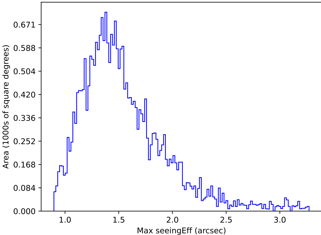
too_5_1v3.4_10yrs Yr 1 g band: Max seeingEff
