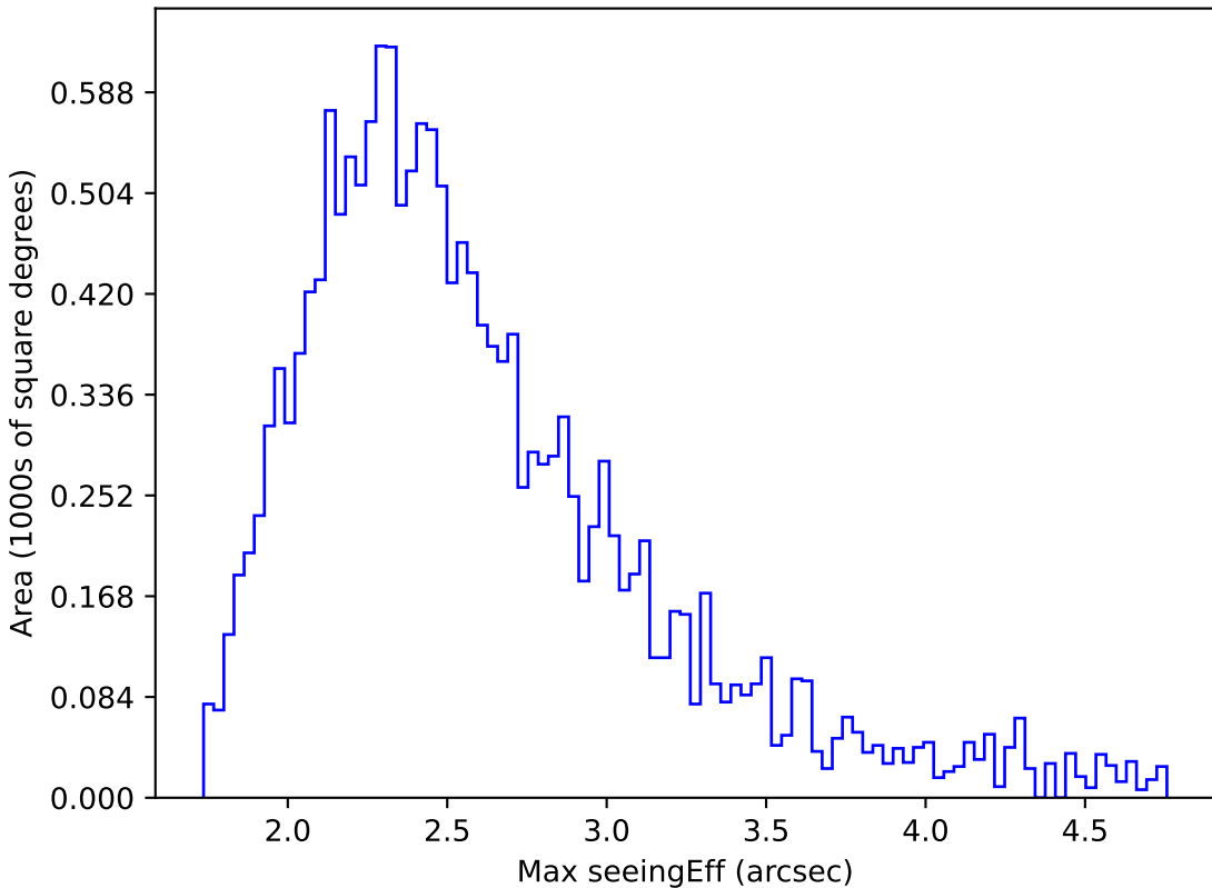
too_5_1v3.4_10yrs WFD z band: Max seeingEff
