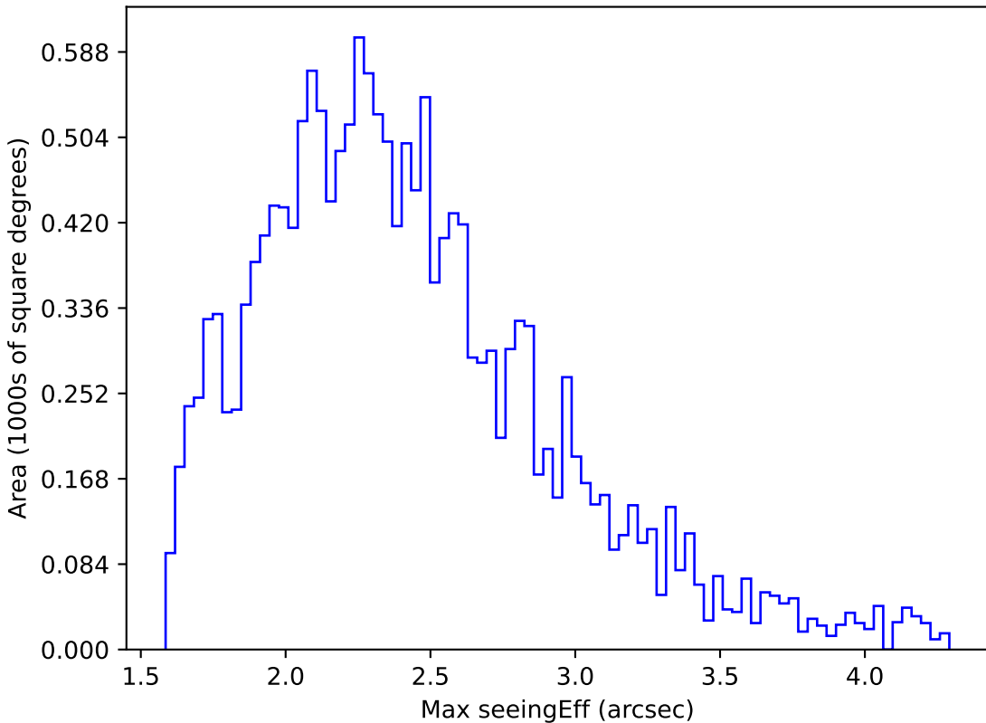
too_5_1v3.4_10yrs WFD y band: Max seeingEff
