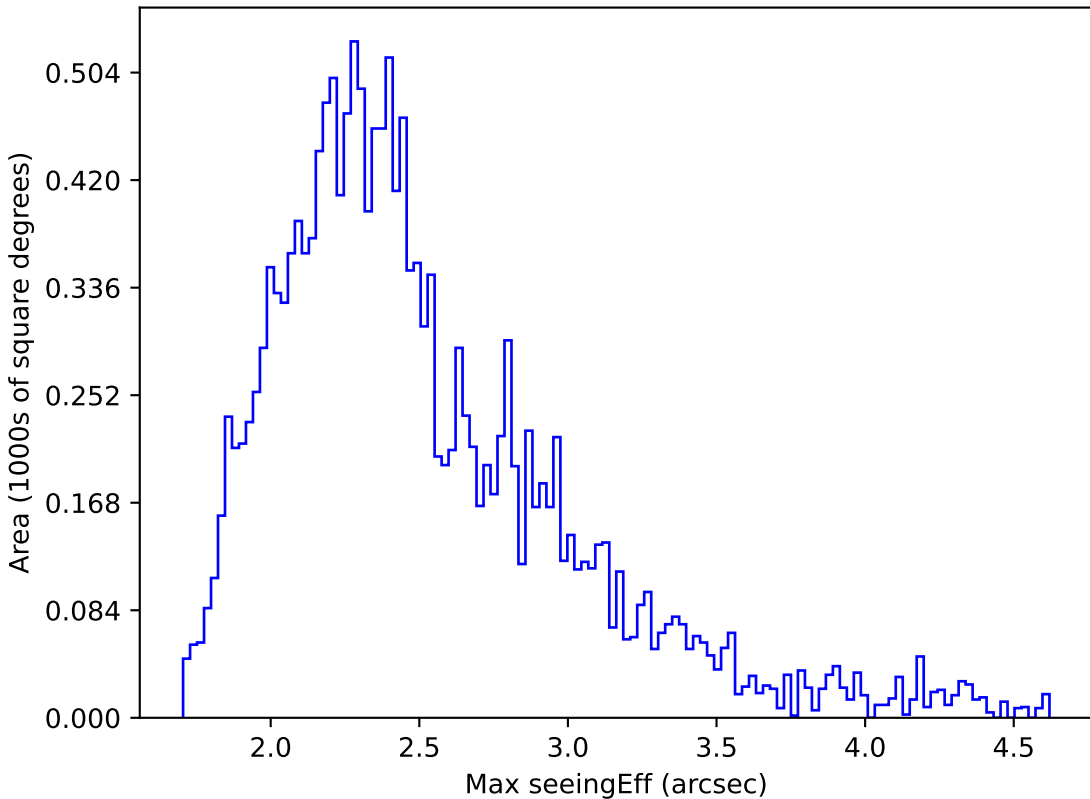
too_5_1v3.4_10yrs WFD u band: Max seeingEff
