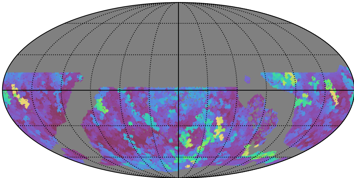
too_5_1v3.4_10yrs WFD i band: Max seeingEff
