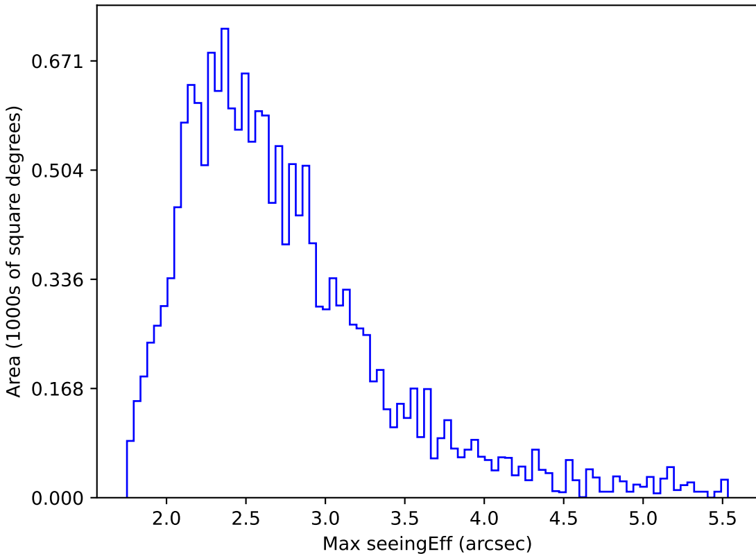
too_5_1v3.4_10yrs WFD i band: Max seeingEff
