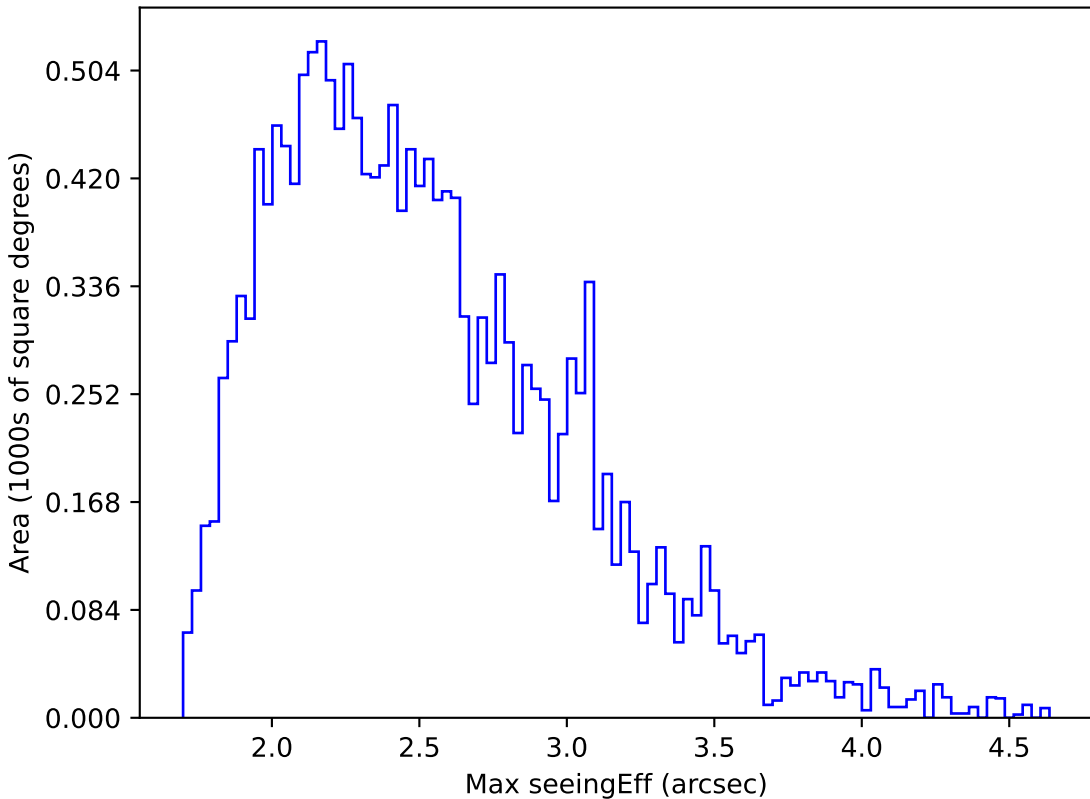
too_5_1v3.4_10yrs WFD g band: Max seeingEff
