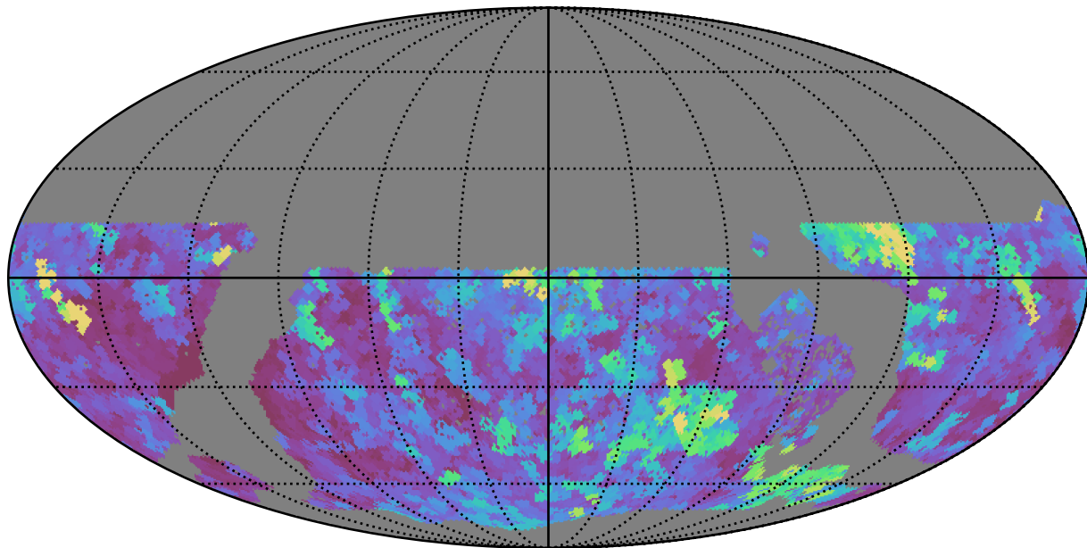
too_5_1v3.4_10yrs WFD all bands: Max seeingEff
