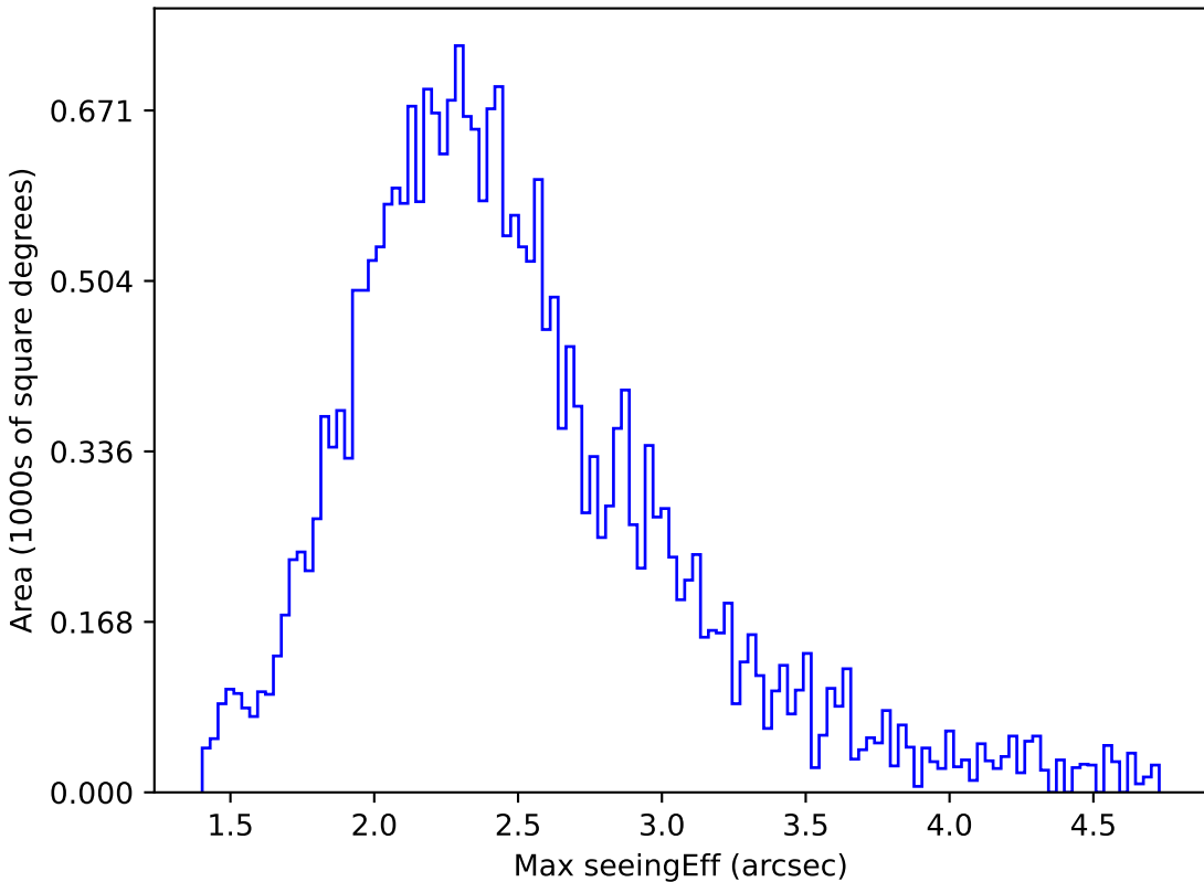
too_5_1v3.4_10yrs All sky z band: Max seeingEff
