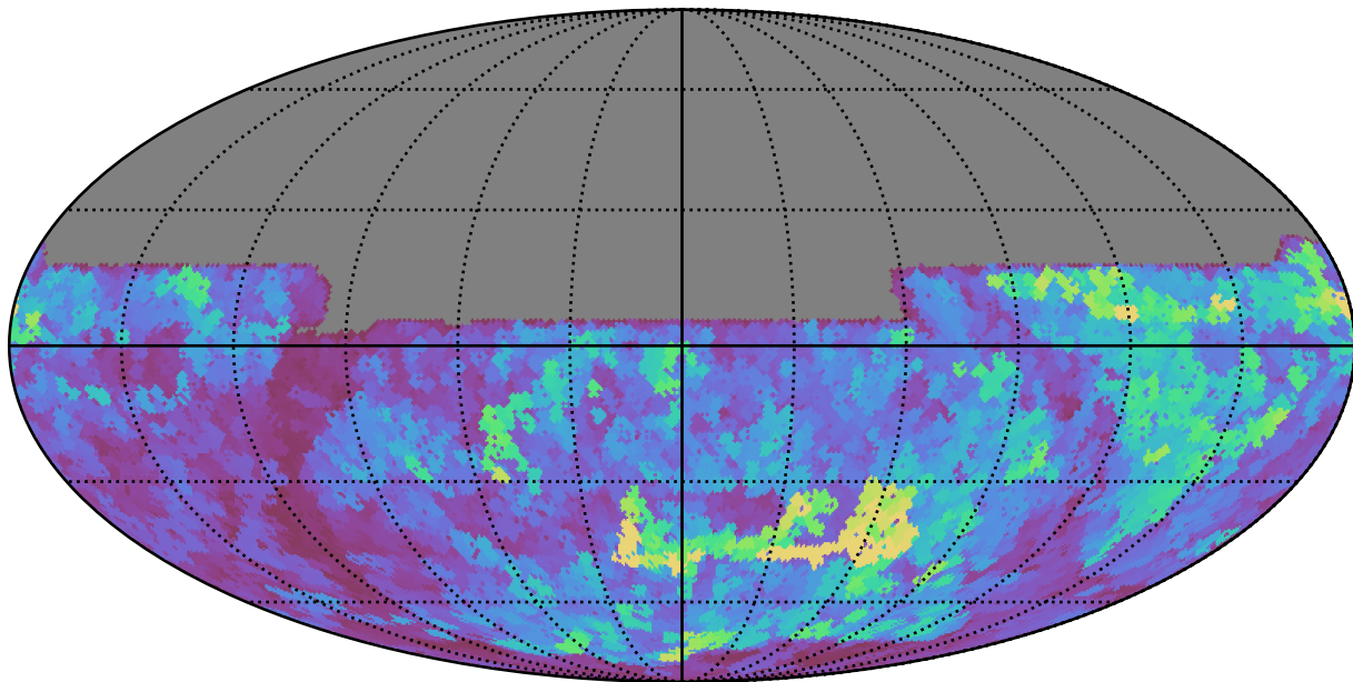
too_5_1v3.4_10yrs All sky y band: Max seeingEff
