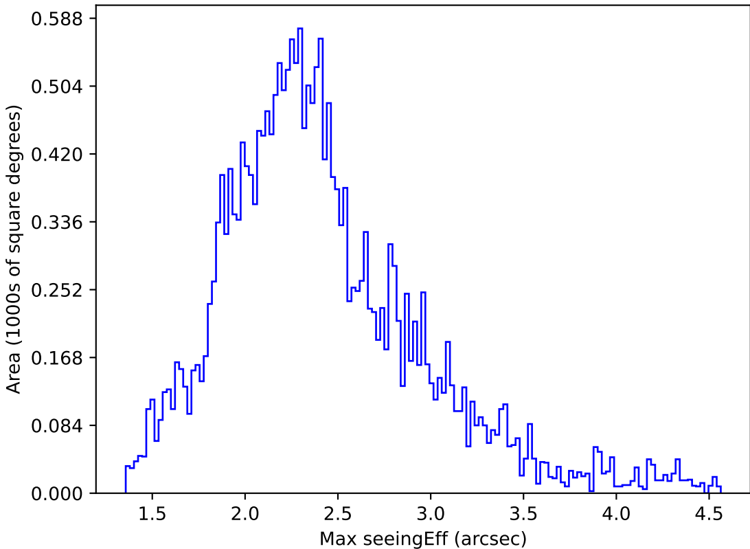
too_5_1v3.4_10yrs All sky u band: Max seeingEff
