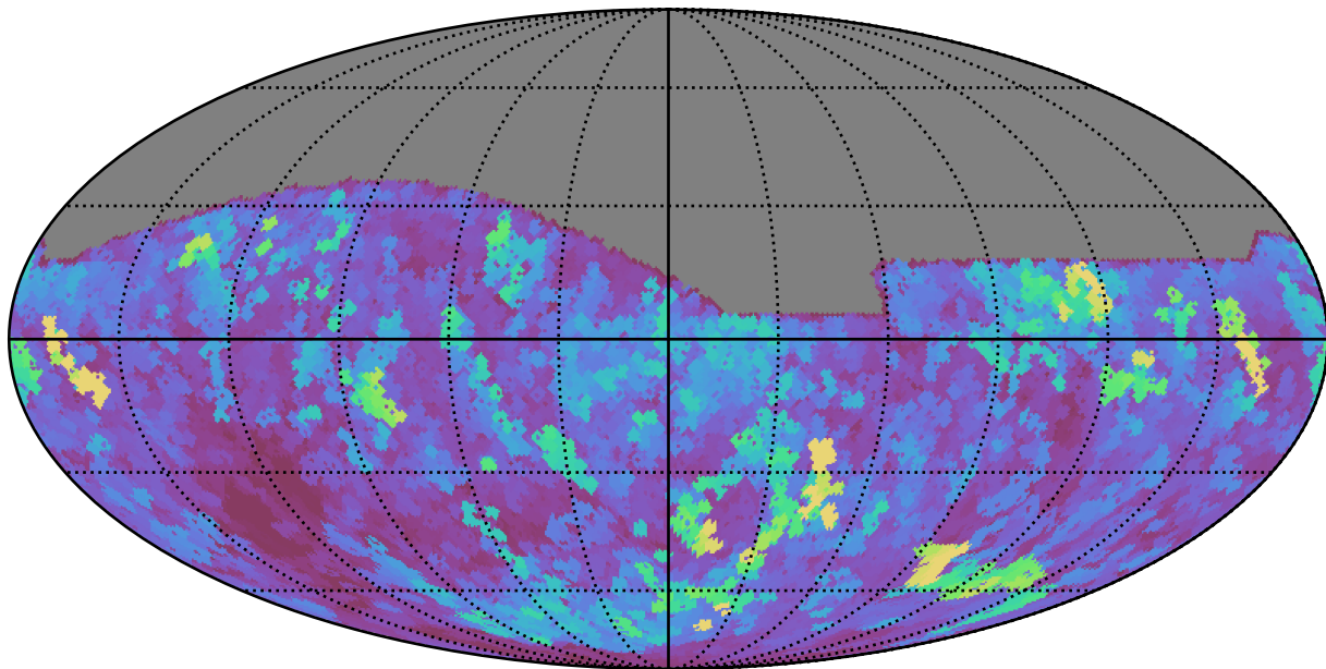
too_5_1v3.4_10yrs All sky i band: Max seeingEff
