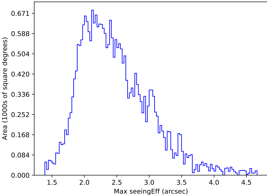
too_5_1v3.4_10yrs All sky g band: Max seeingEff
