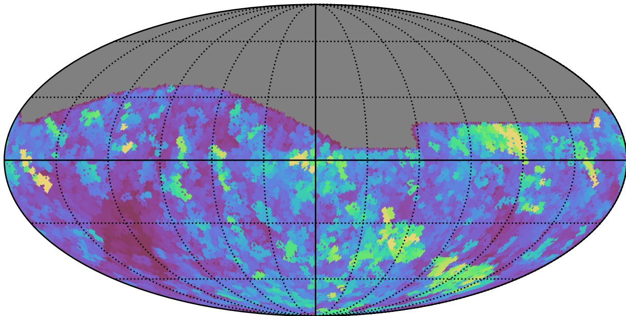
too_5_1v3.4_10yrs All sky all bands: Max seeingEff
