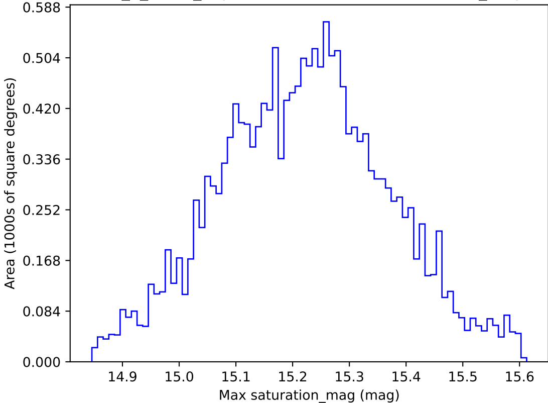
too_5_1v3.4_10yrs WFD z band: Max saturation_mag
