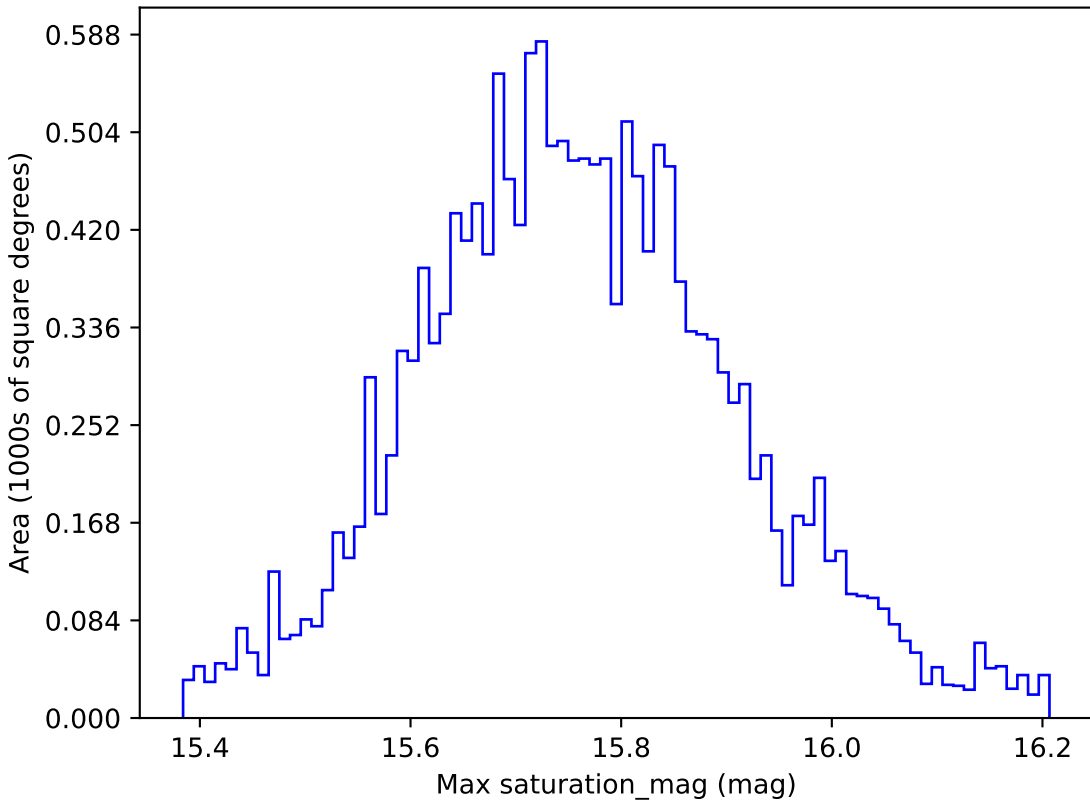
too_5_1v3.4_10yrs WFD r band: Max saturation_mag
