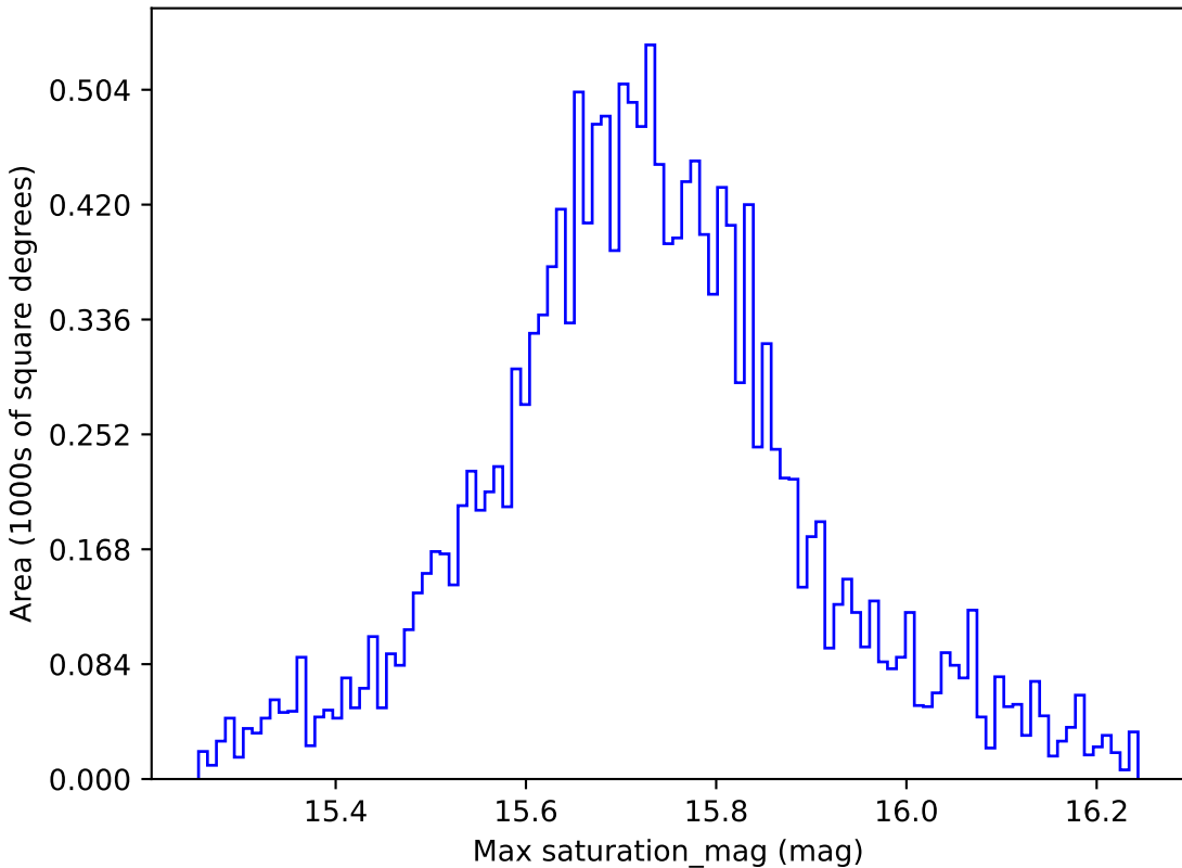
too_5_1v3.4_10yrs WFD g band: Max saturation_mag
