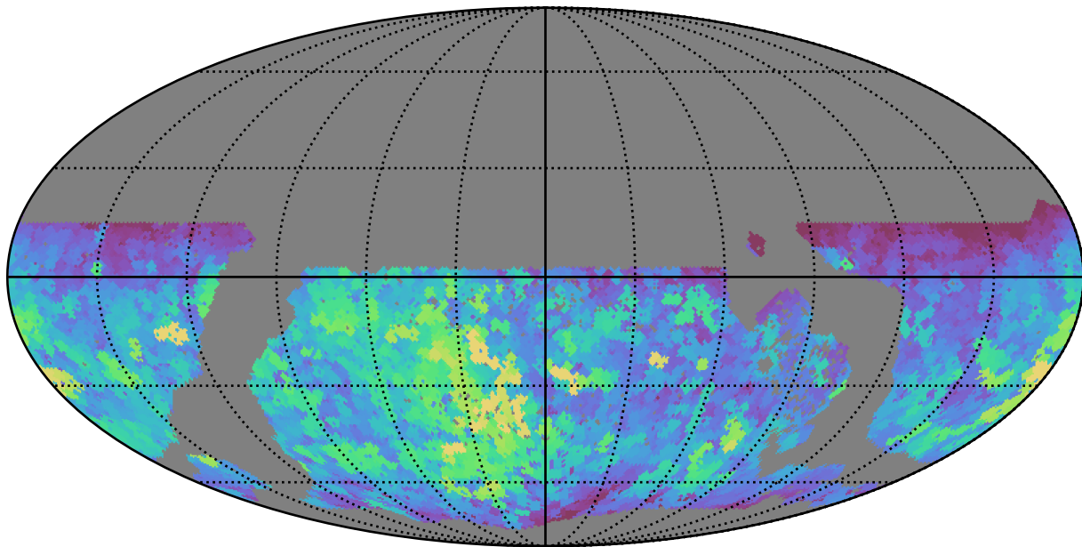
too_5_1v3.4_10yrs WFD all bands: Max saturation_mag
