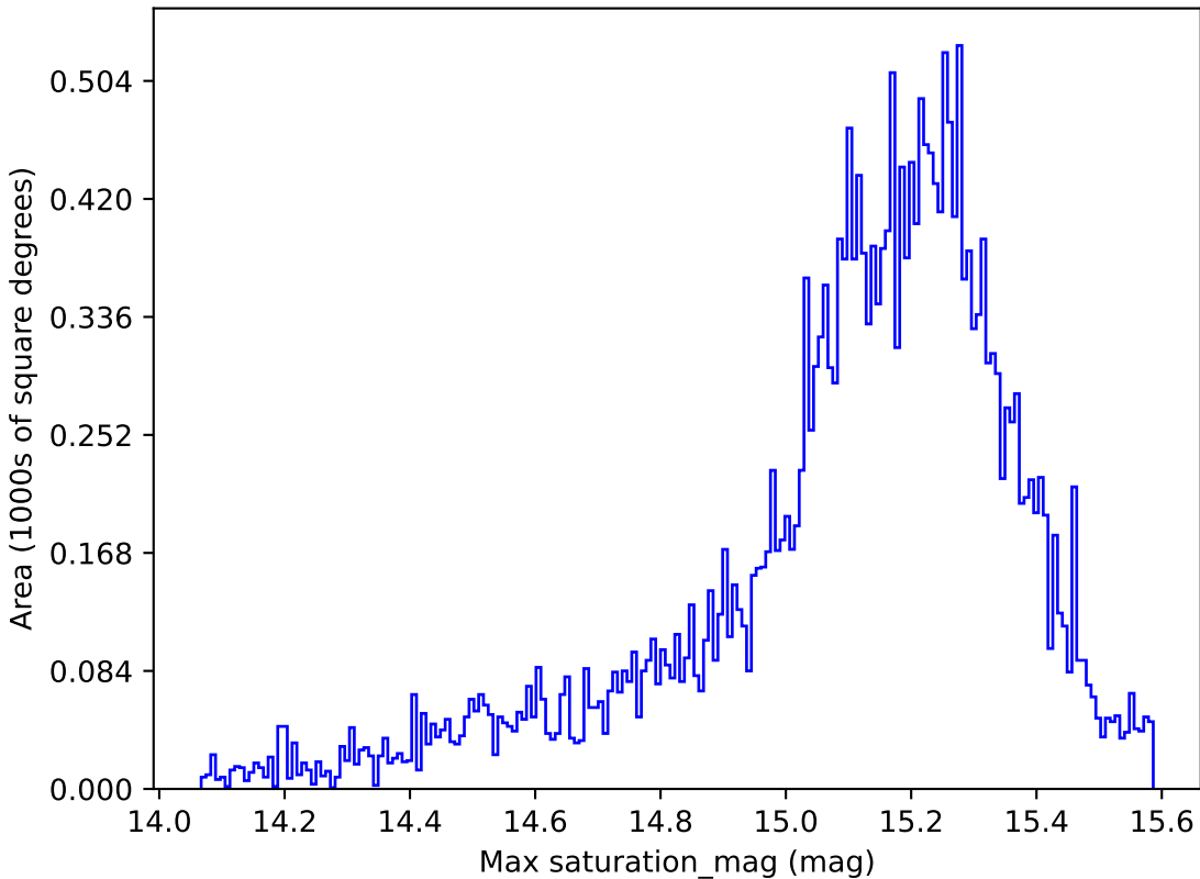
too_5_1v3.4_10yrs All sky z band: Max saturation_mag
