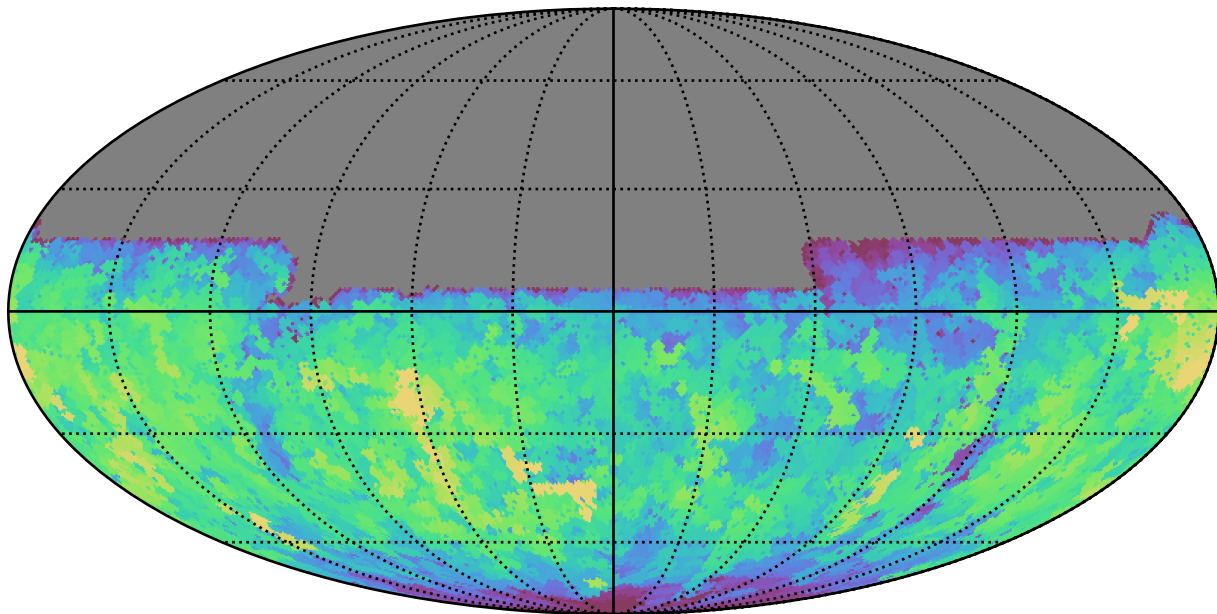
too_5_1v3.4_10yrs All sky u band: Max saturation_mag
