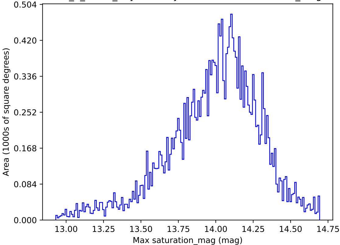
too_5_1v3.4_10yrs All sky u band: Max saturation_mag
