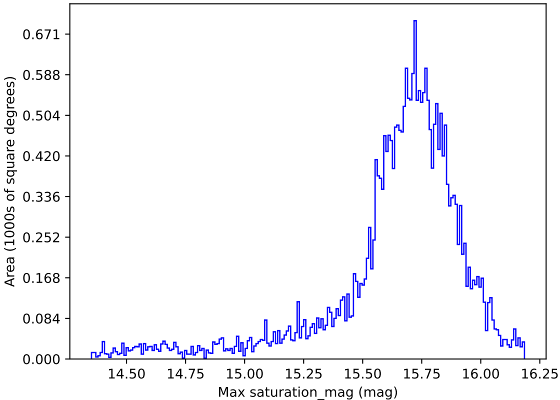
too_5_1v3.4_10yrs All sky r band: Max saturation_mag
