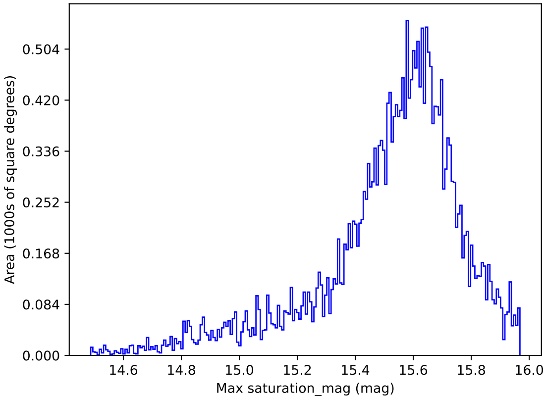
too_5_1v3.4_10yrs All sky i band: Max saturation_mag
