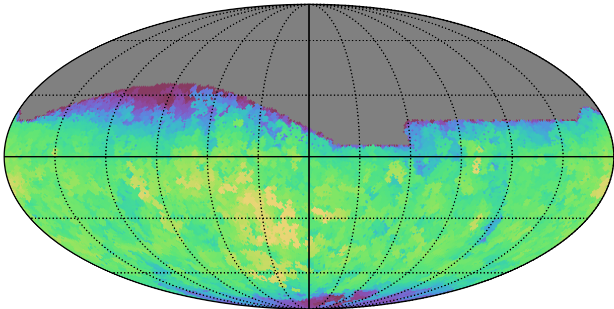
too_5_1v3.4_10yrs All sky g band: Max saturation_mag
