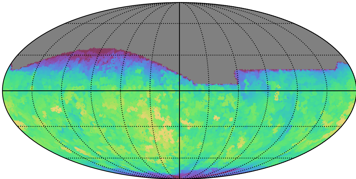
too_5_1v3.4_10yrs All sky all bands: Max saturation_mag
