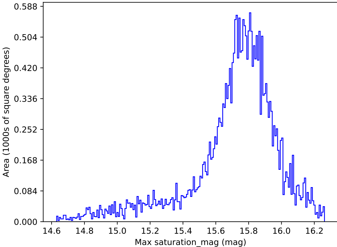
too_5_1v3.4_10yrs All sky all bands: Max saturation_mag
