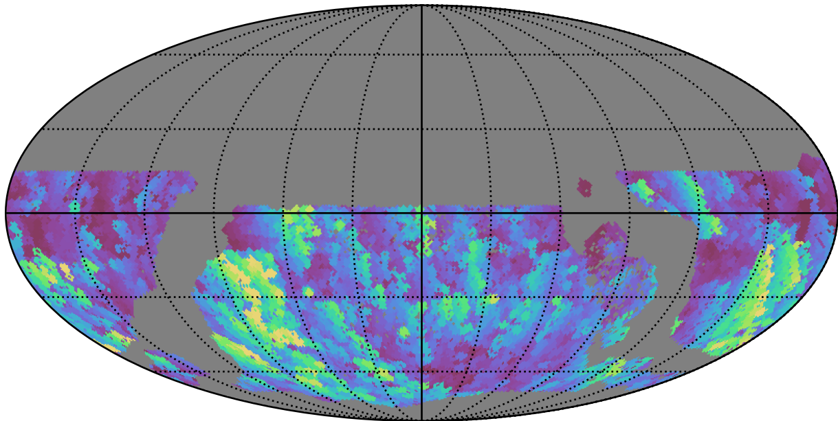
too_5_1v3.4_10yrs WFD u band: Max normairmass
