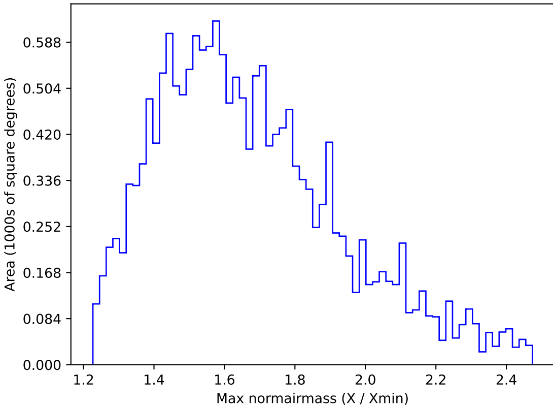
too_5_1v3.4_10yrs WFD u band: Max normairmass
