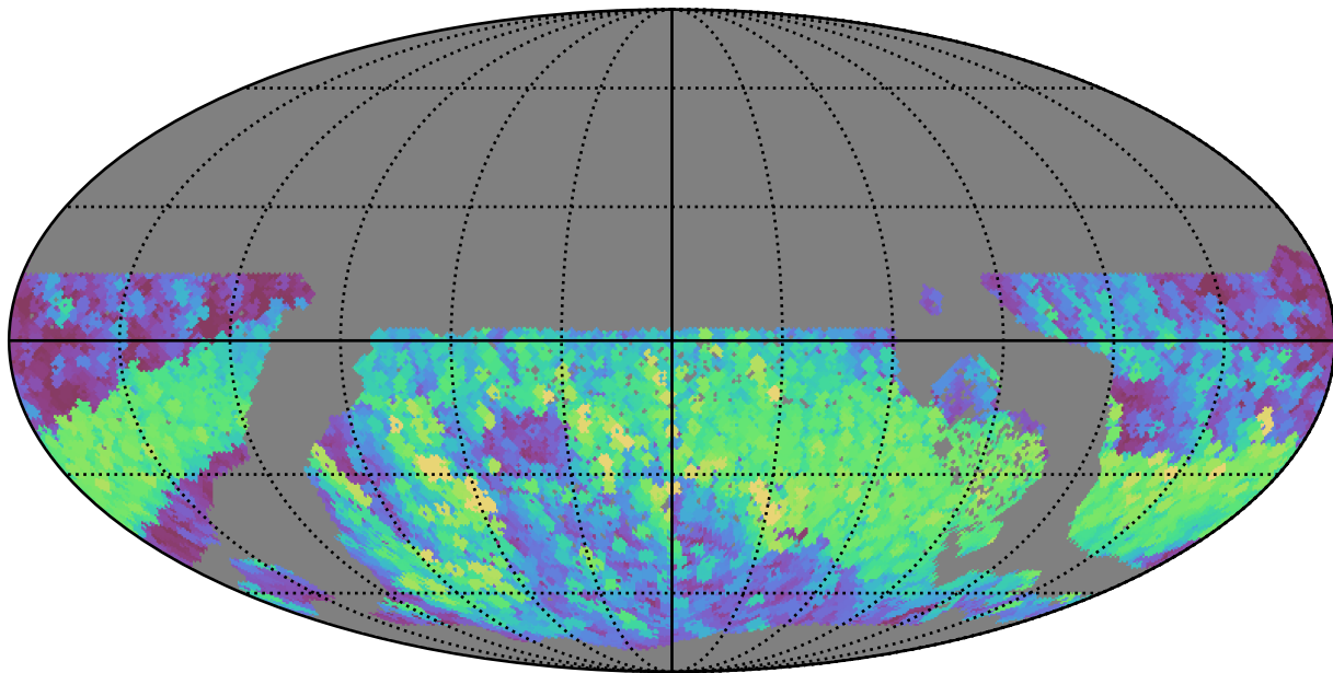
too_5_1v3.4_10yrs WFD r band: Max normairmass
