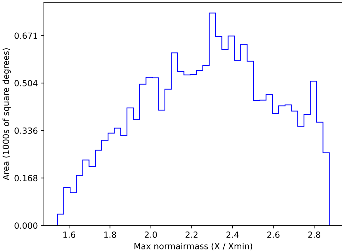
too_5_1v3.4_10yrs WFD i band: Max normairmass
