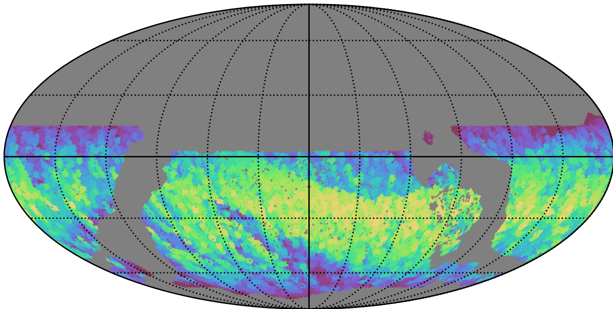
too_5_1v3.4_10yrs WFD all bands: Max normairmass
