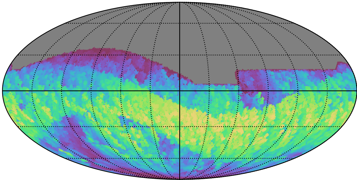
too_5_1v3.4_10yrs All sky z band: Max normairmass
